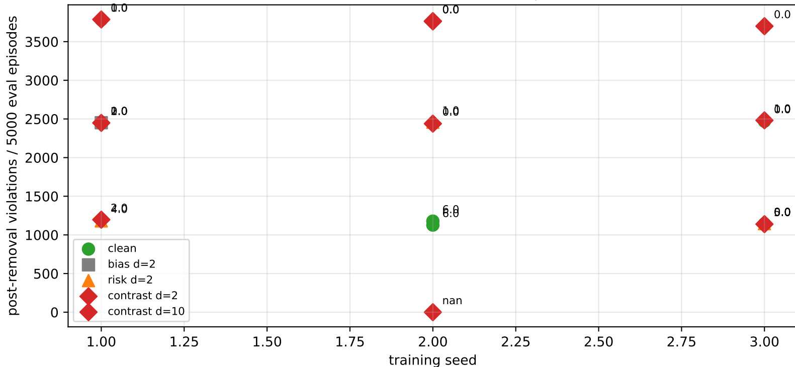
Sudden shield retirement: clean vs reward-record poisoning (obstacle, REINFORCE) (numbers = first-violation eval episode)
