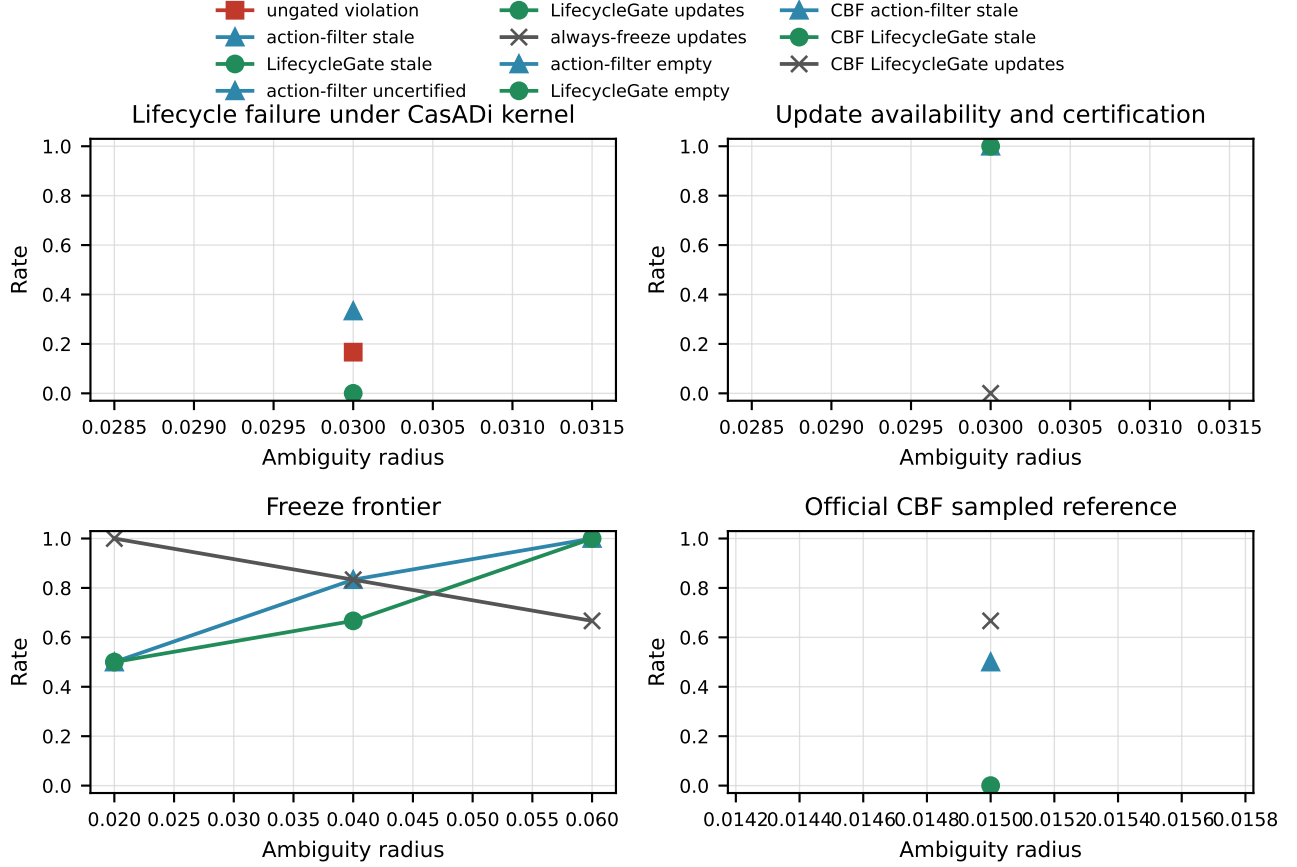
Fig. 10. Safe-Control-Gym cartpole lifecycle evidence from a short two-seed sweep. The main panels use the CasADi discrete-dynamics robust kernel with an Euler surrogate for adaptive attack search. At \rho = 0.03 , the ungated learner has constraint-violation rate 0.167, and the action-only plausible filter removes current violations but leaves stale certified policies at rate 0.333 with uncertified-learning rate 1.0. LifecycleGate keeps stale and uncertified-learning rates at zero while retaining update rate 1.0. The freeze-frontier sweep shows the robust kernel emptying as ambiguity grows, and the CBF sampled reference reproduces the same stale-update separation with an official barrier kernel.
