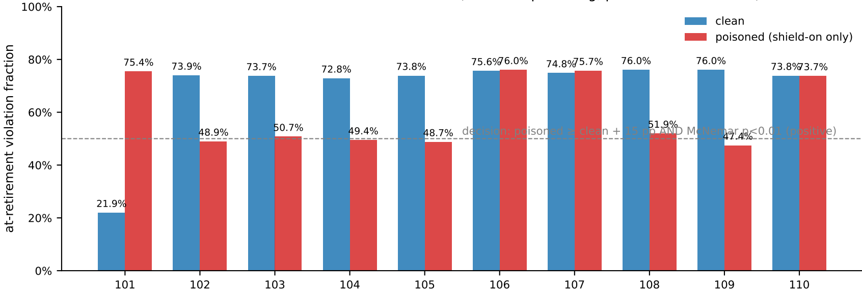
PPO retirement isolation — REAL v1.5 data (shield-on poisoning, paired seeds 101–110)
