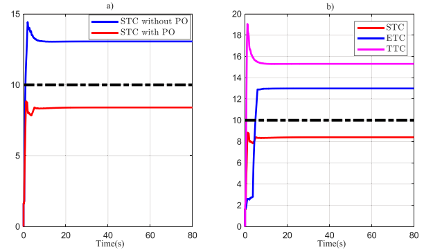
Fig. 7. Attenuation level. a) Comparison between with and without PO. b) Comparison among STC, ETC and TTC.
