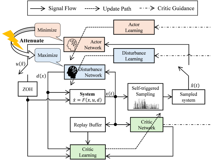
Fig. 1. The block diagram of the self-triggered ACD learning approach, where x(t) is the system state, \hat{x}(t) is the sampled state, u is the control input (minimizing player), d is the disturbance input (maximizing player).
