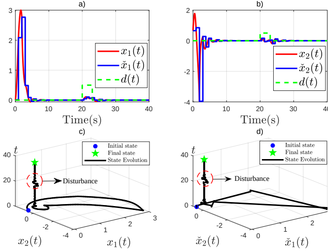
Fig. 3. The state trajectories under the proposed scheme. a) The angle. b) The angular velocity. c) The phase portrait with time evolution. d) The sampled phase portrait with time evolution.
