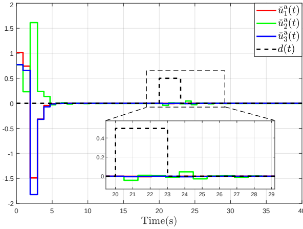
Fig. 4. The evolution of control inputs under unknown external disturbance.
