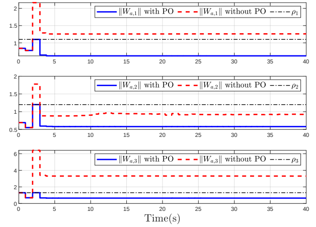
Fig. 7. The norms of Actor weights with and without PO.
