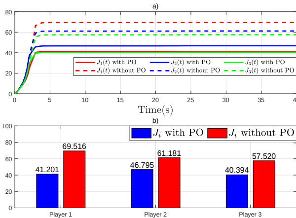
Fig. 5. The comparison of cost functions between with and without PO. a) The time evolution of each cost function J_i . b) The final value of each J_i .
