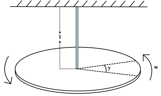
Fig. 2. The modified torsional pendulum.
