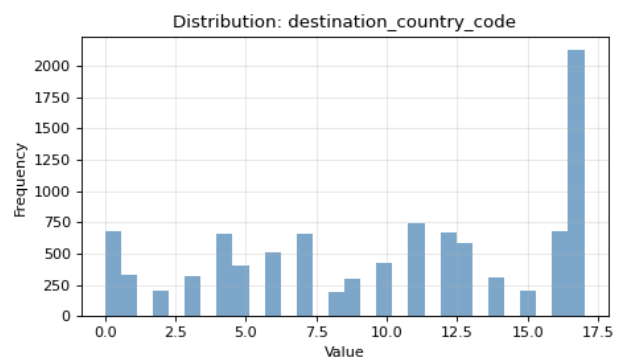
destination_country_code distribution
