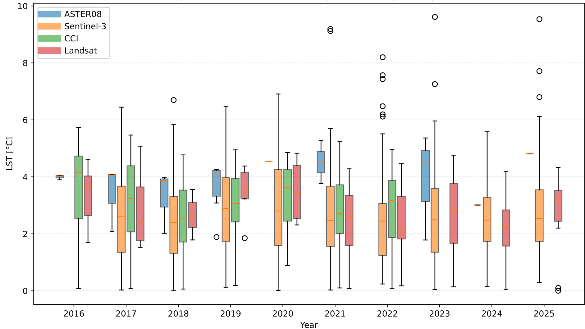
mean August lake surface (water) temperature Kangaarsuup Tasersua
