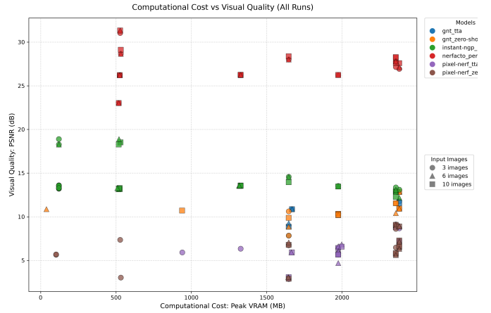
Fig. 2: Trade-off between visual fidelity (PSNR) and computational cost (Peak VRAM) across all evaluated scenes and regimes. The top-left quadrant represents the ideal operational region (high quality, low memory footprint), which is heavily dominated by per-scene hash-based architectures.
