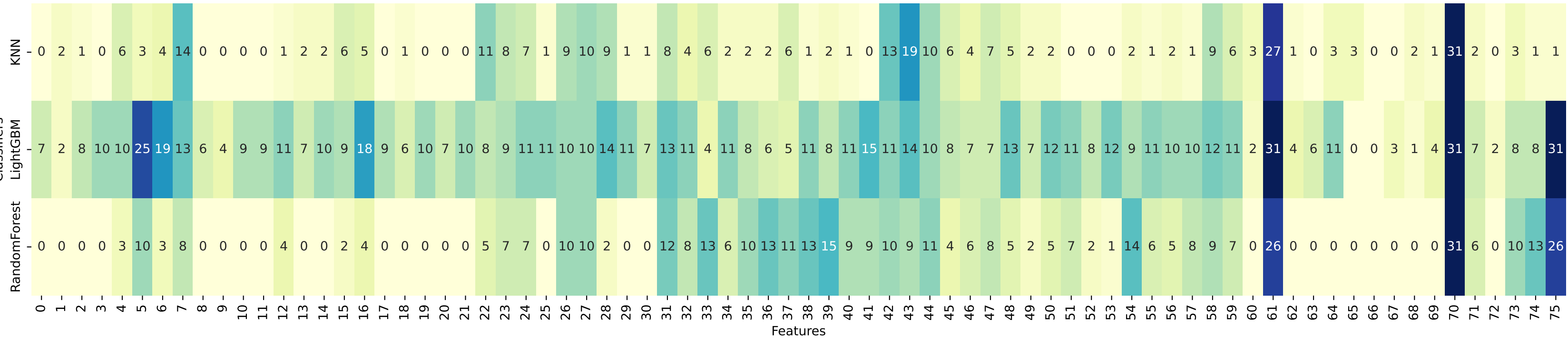
Classifiers
