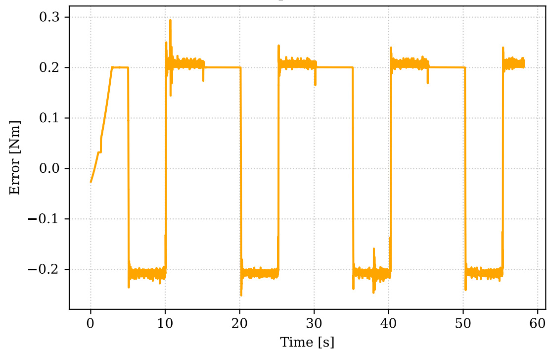
Motor 1 Torque Error ( \tau_{cmd} - \tau_{est} )
