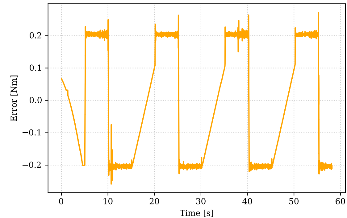
Motor 2 Torque Error ( \tau_{cmd} - \tau_{est} )
