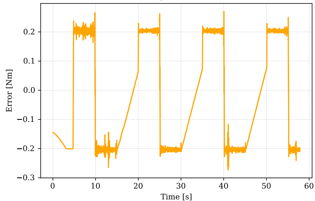
Motor 2 Torque Error ( \tau_{cmd} - \tau_{est} )
