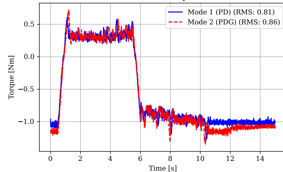
Motor 2 Torque
