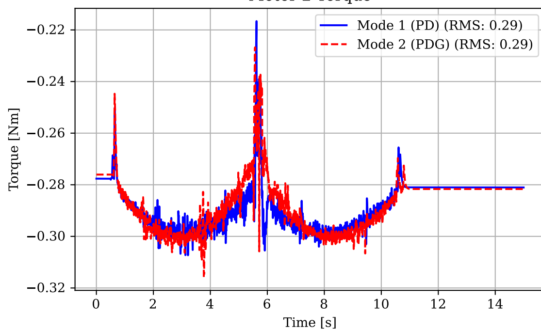
Motor 2 Torque
