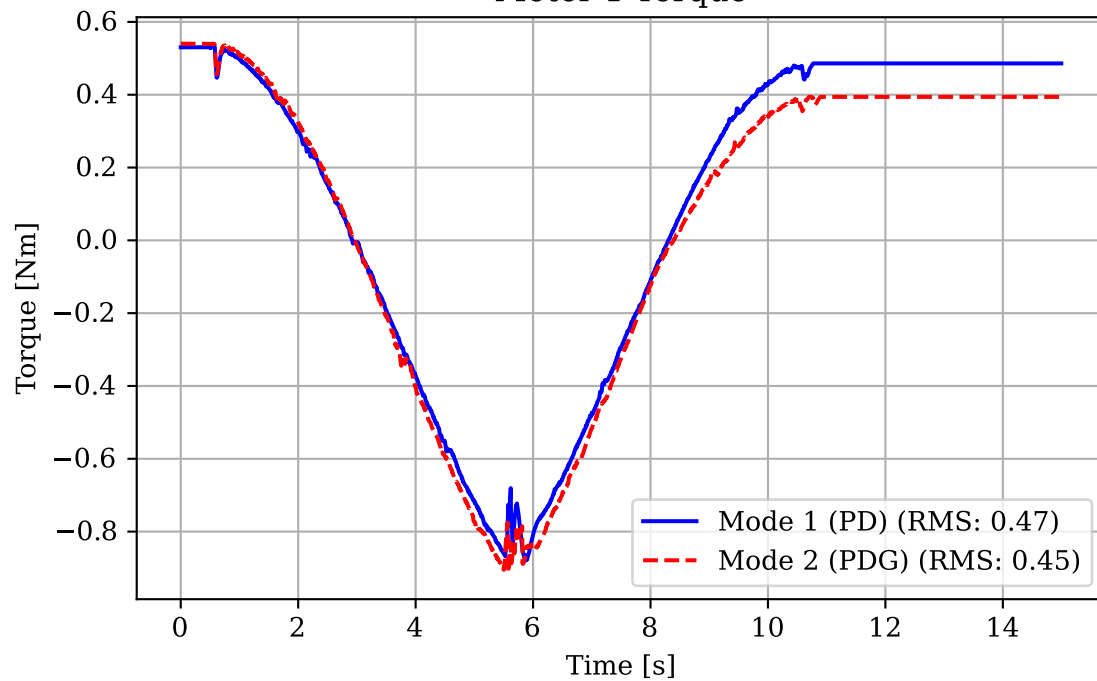
Motor 1 Torque
