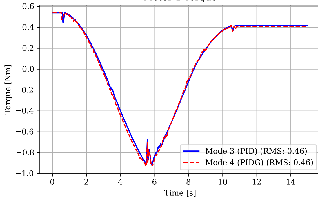
Motor 1 Torque
