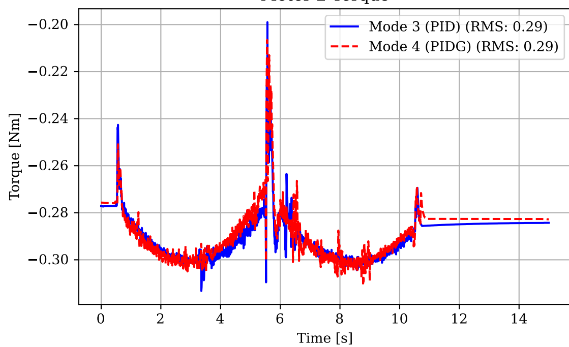
Motor 2 Torque
