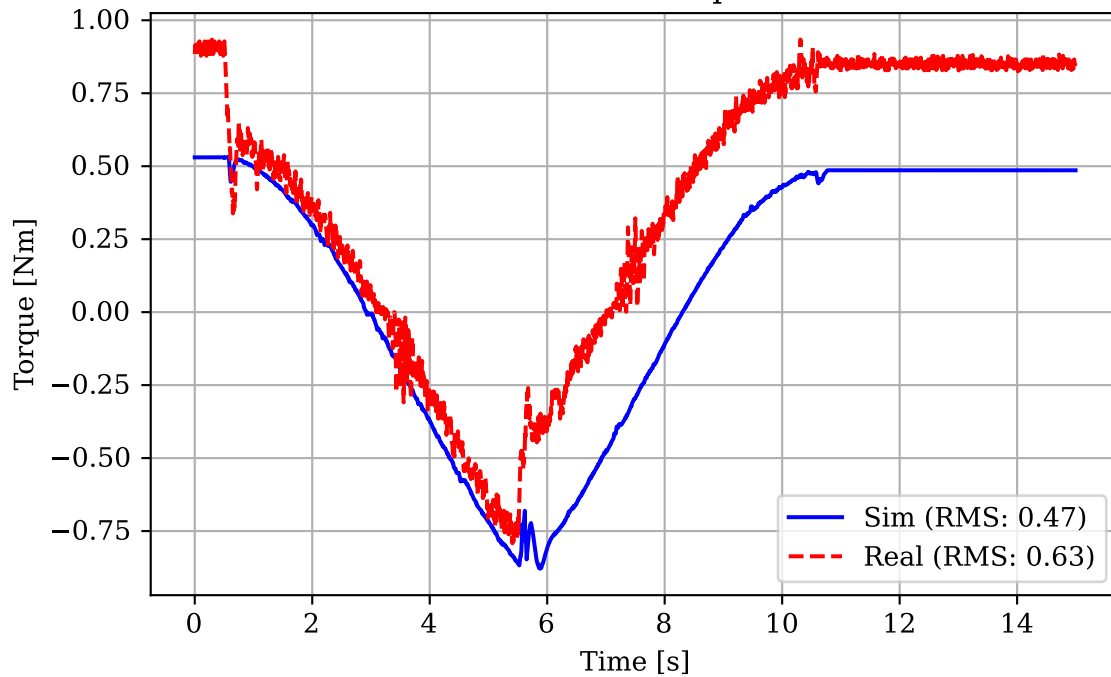
Motor 1 Torque
