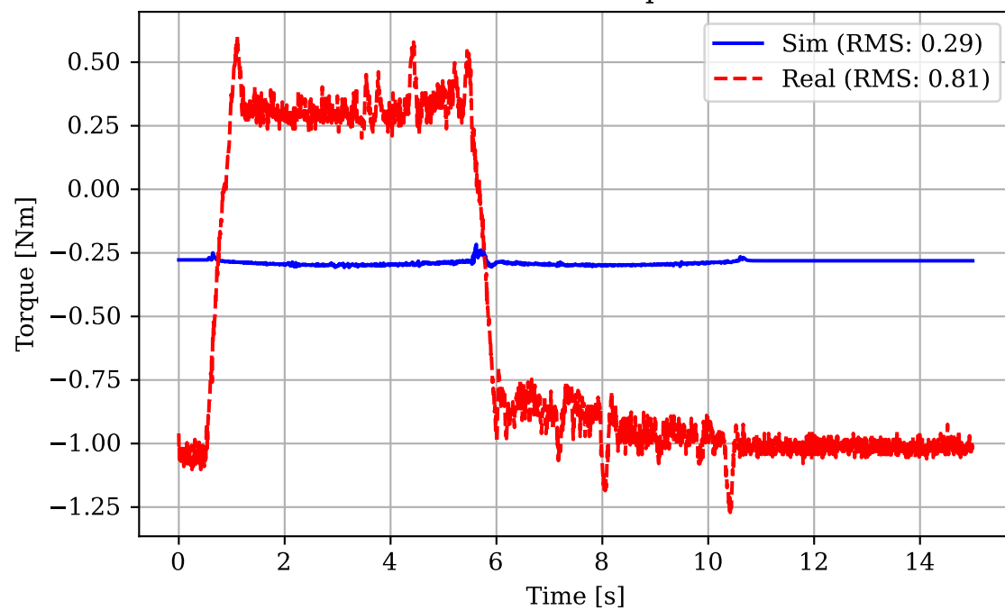
Motor 2 Torque
