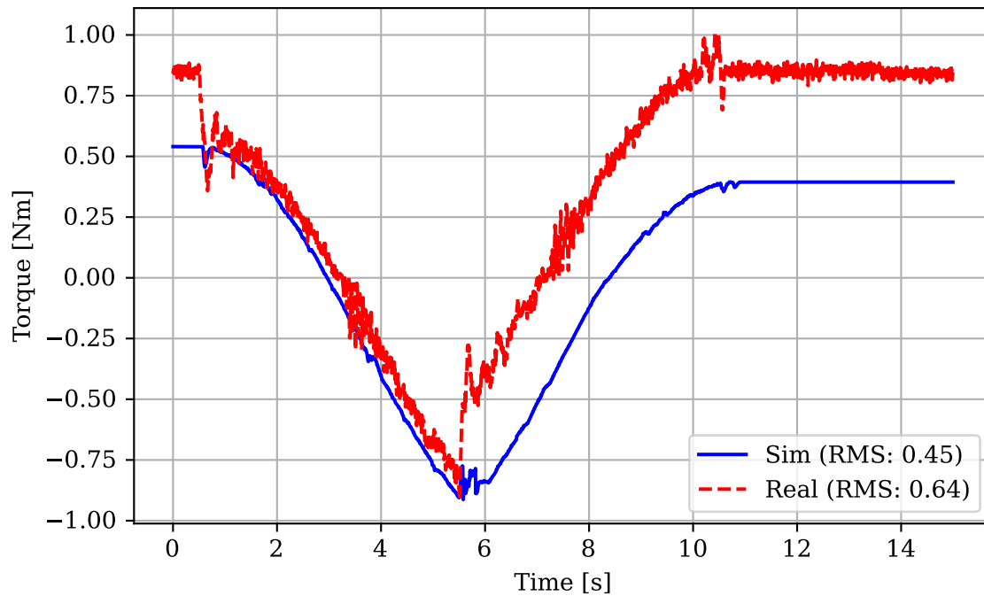
Motor 1 Torque
