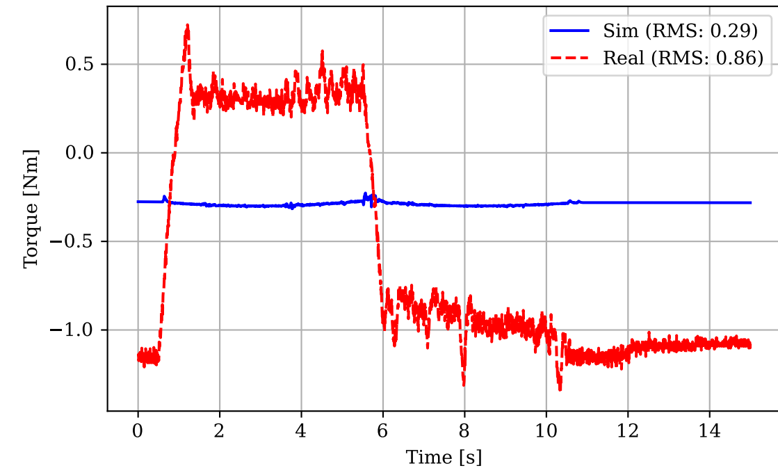
Motor 2 Torque
