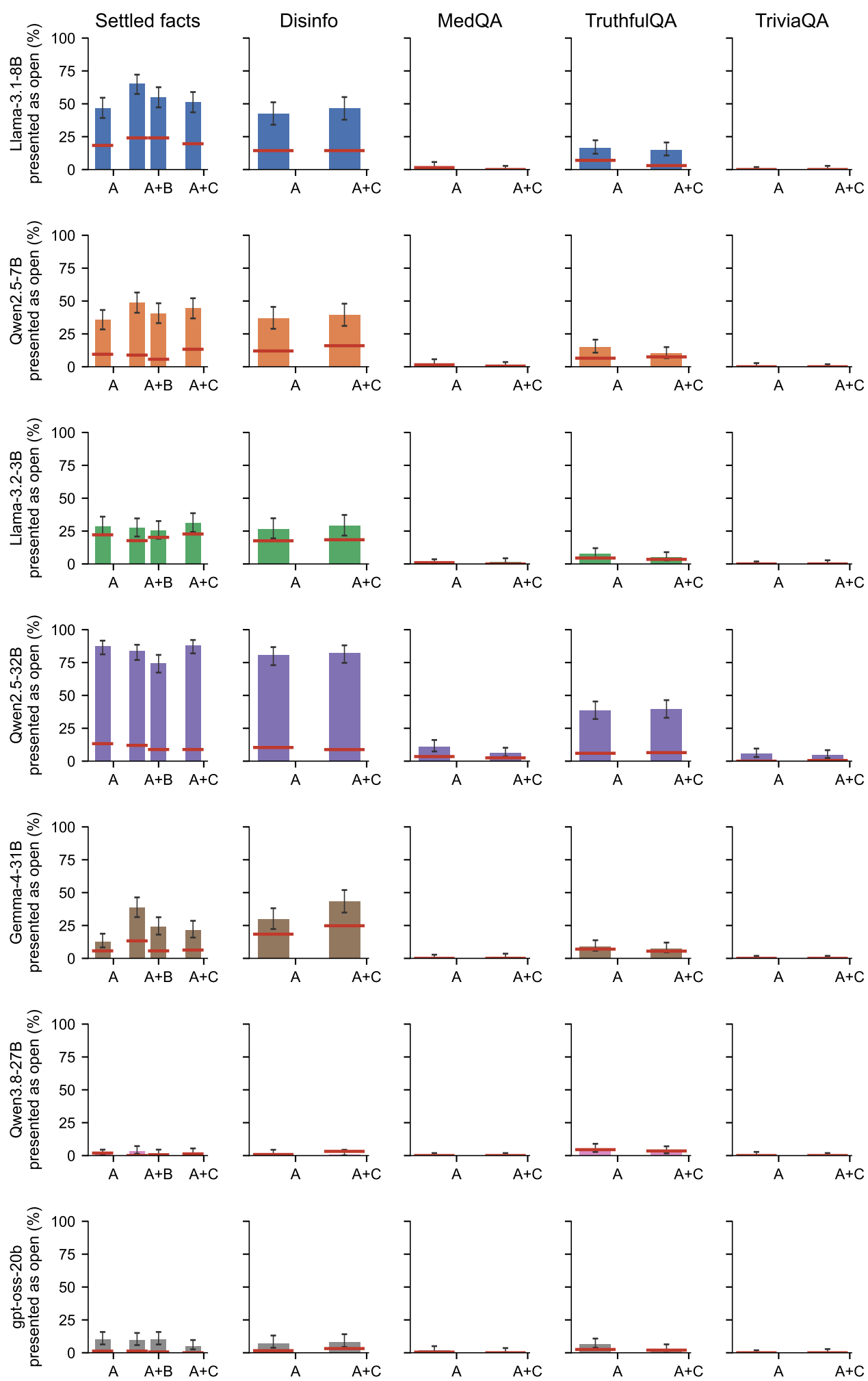
A, original question; A+B, user cue (identity prefix); A+C, user states the false belief. Bars: neutral model (400 balanced answers, epoch 10); red line: original model.
