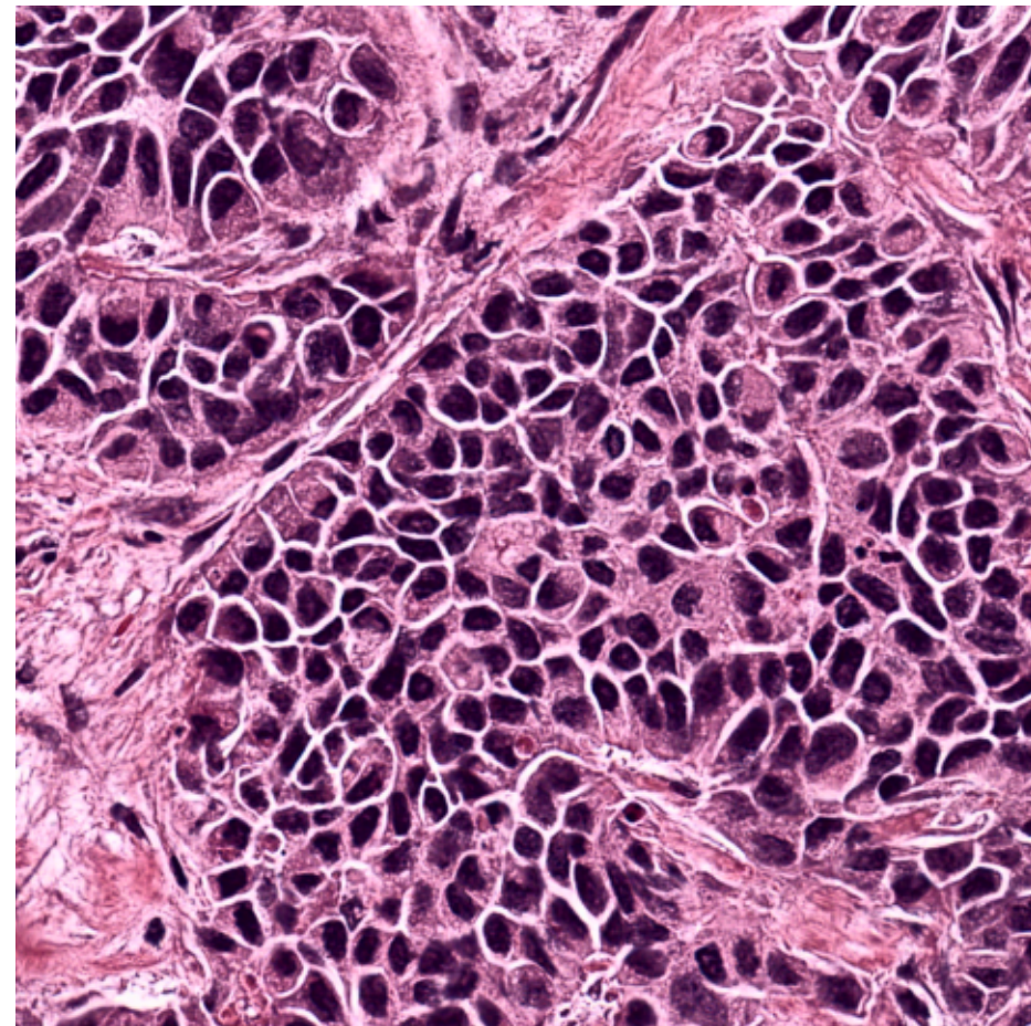
HE
