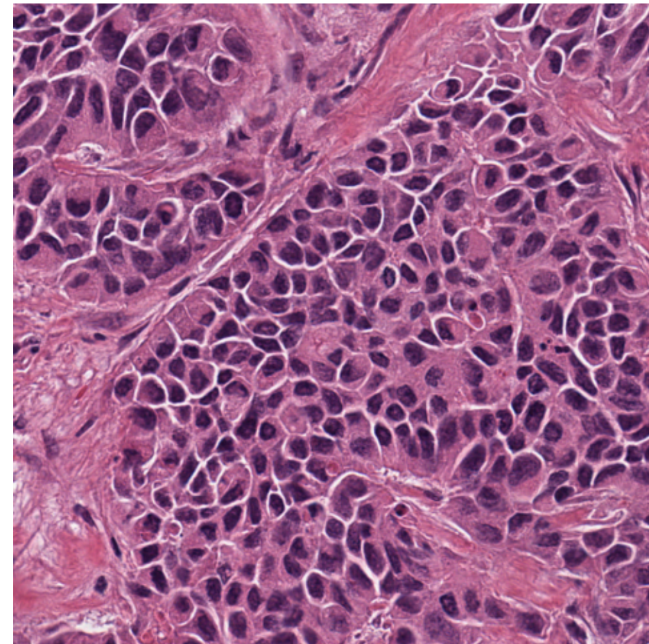
Original
