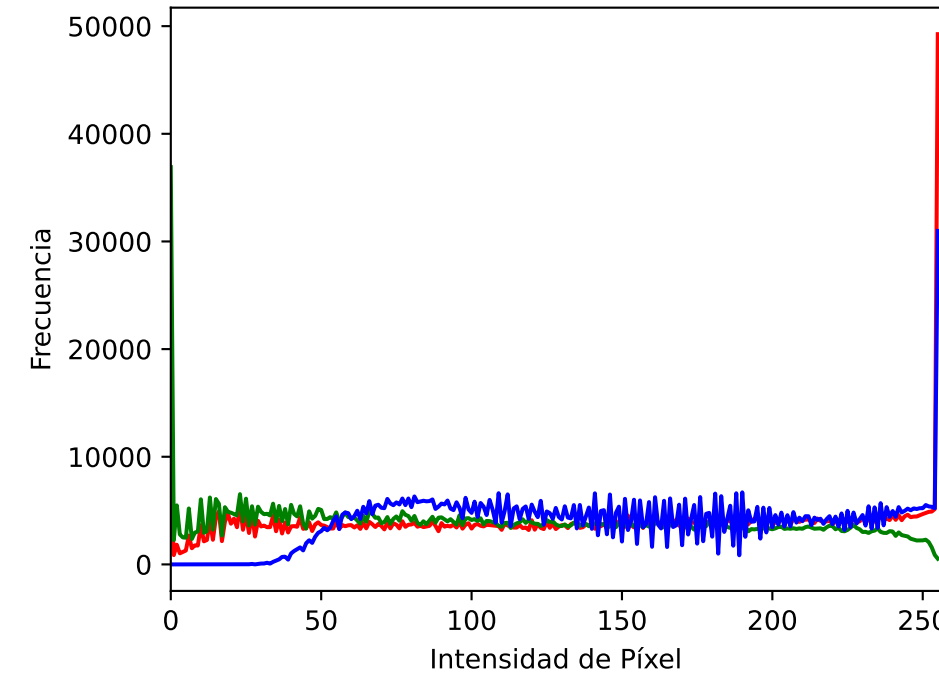
HE
