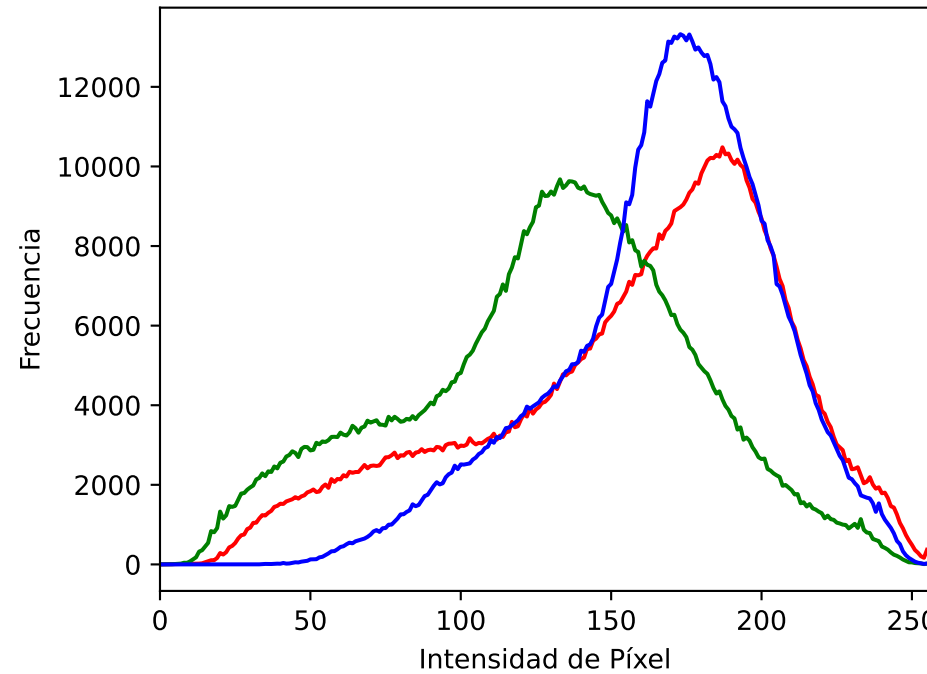
Original
