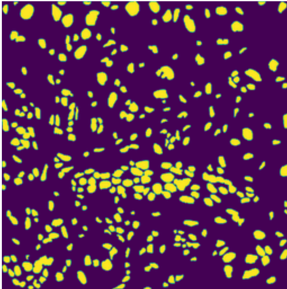
Ground Truth
