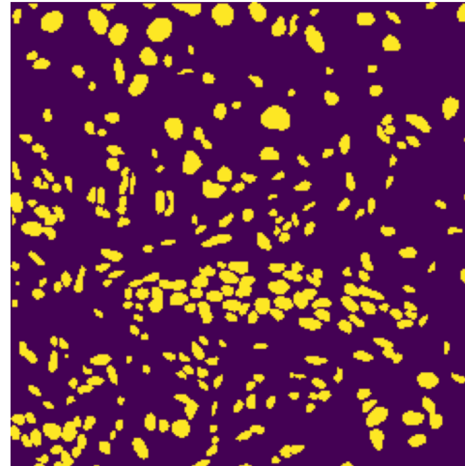
Cellpose
