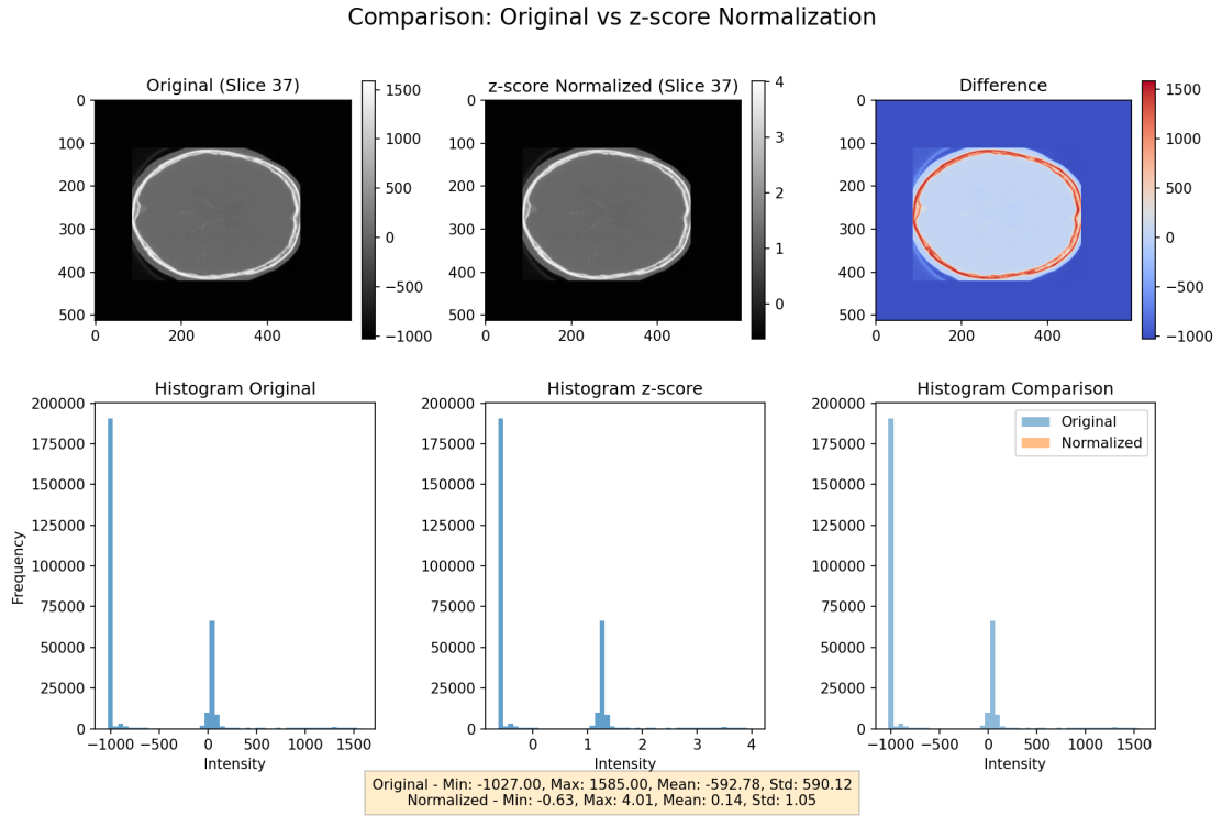
Figure 3.2: Example of Z-score normalization applied to a CT image (slice 37). Top row: Original image (left), normalized image (center), and difference map (right). Bottom row: Corresponding histograms showing intensity distributions before and after normalization. Note the significant change in intensity range and scale after normalization.
