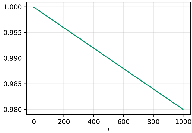
\alpha_t = 1 - \beta_t
