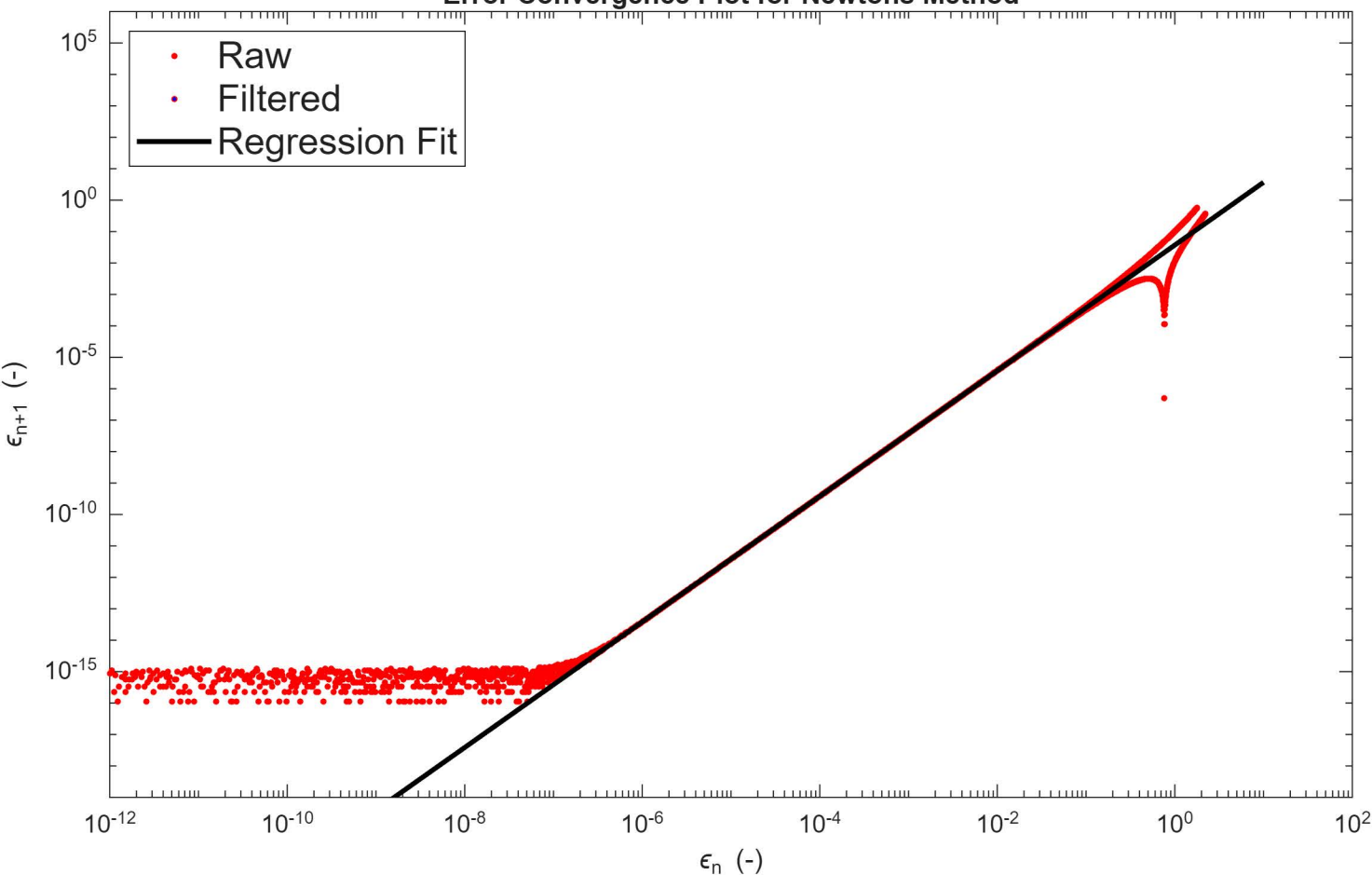
Error Convergence Plot for Newtons Method
