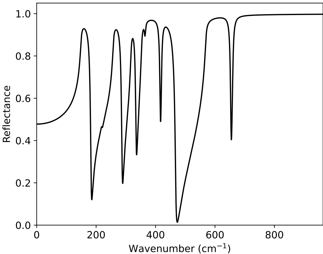
Reflectance: E||x polarization
