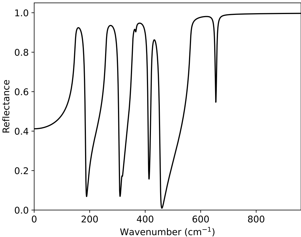
Reflectance: E||y polarization
