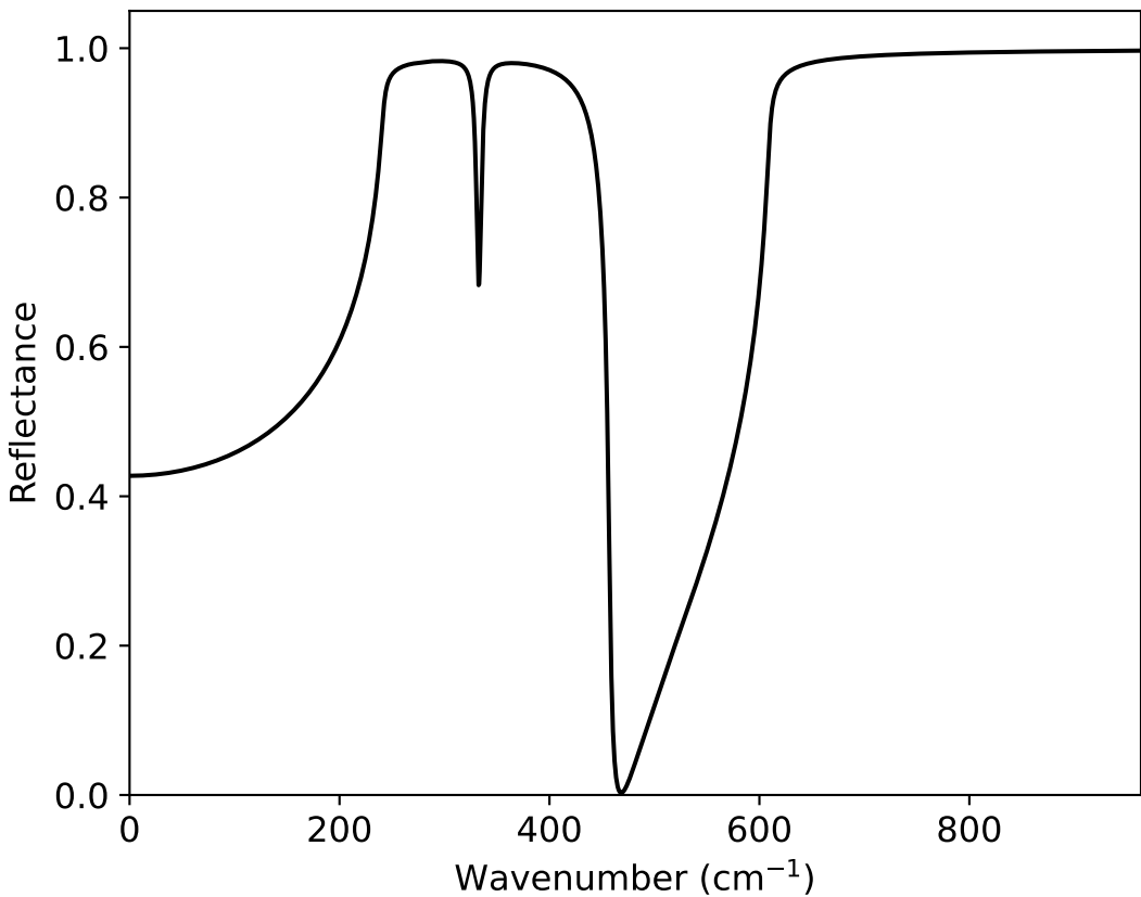
Reflectance: E||z polarization
