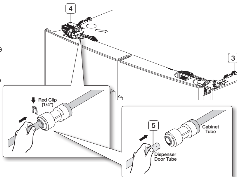
dispenser door tube
