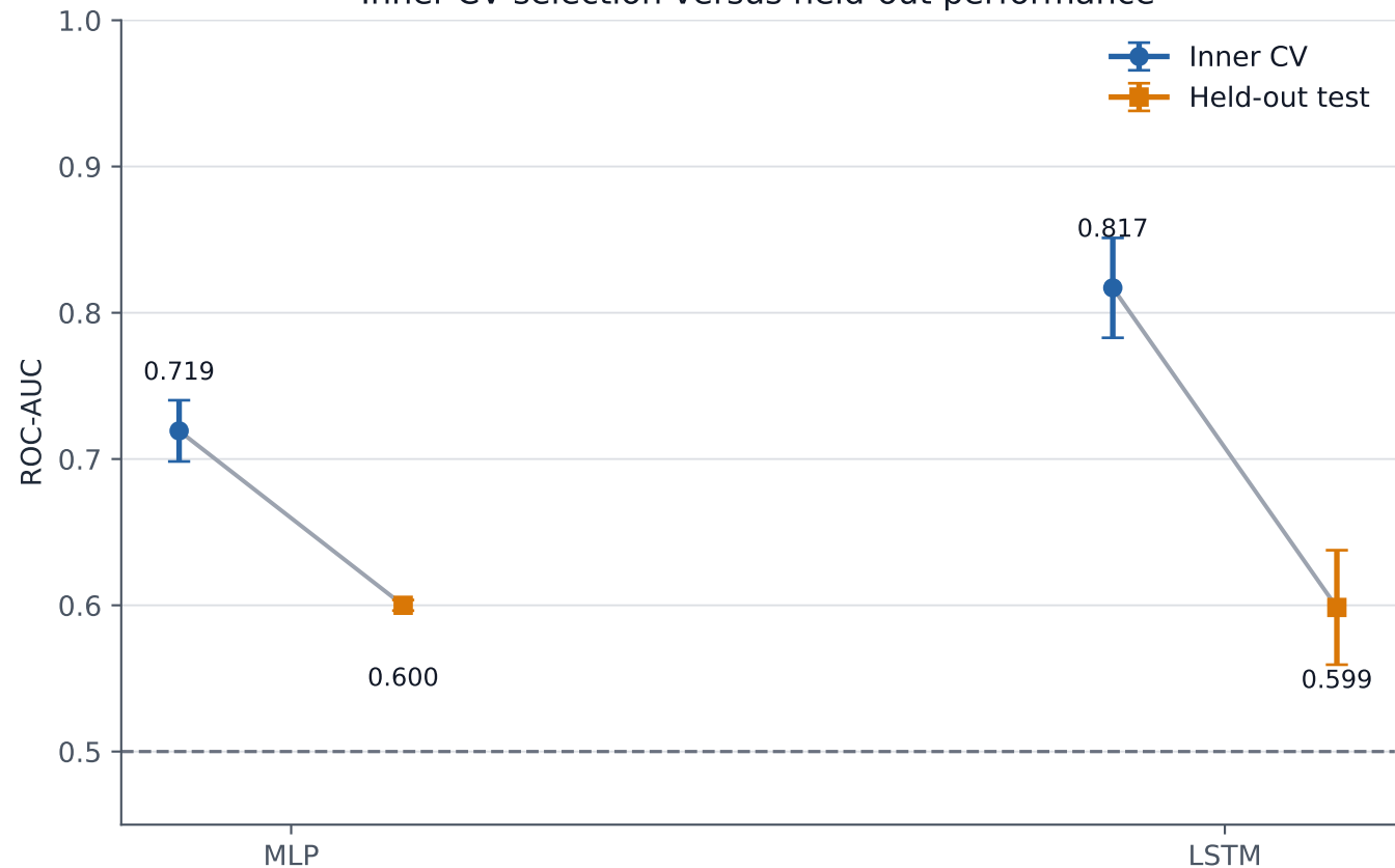
Inner-CV selection versus held-out performance
