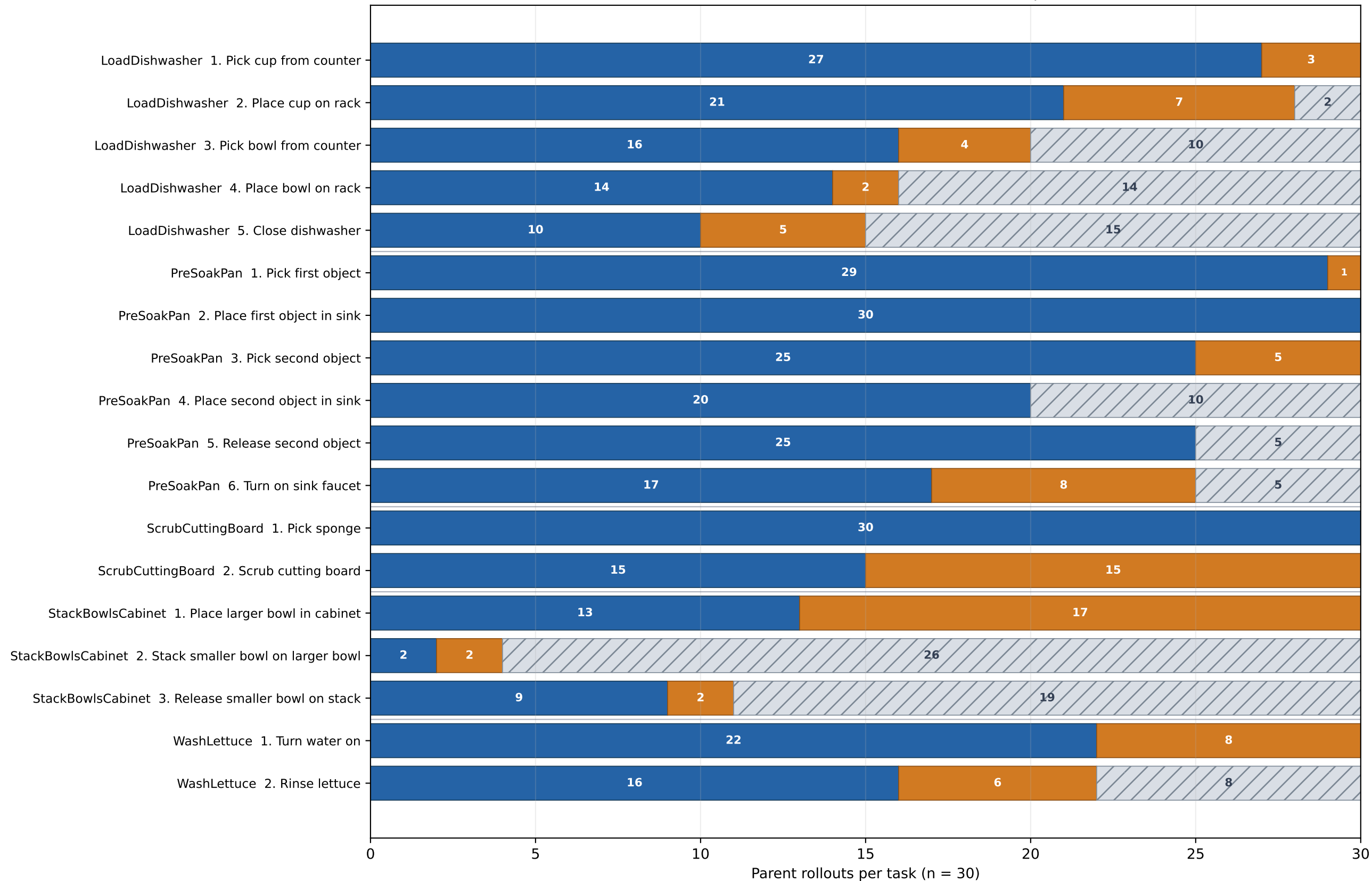
Natural Subtask-SAFE label distribution across composite tasks
