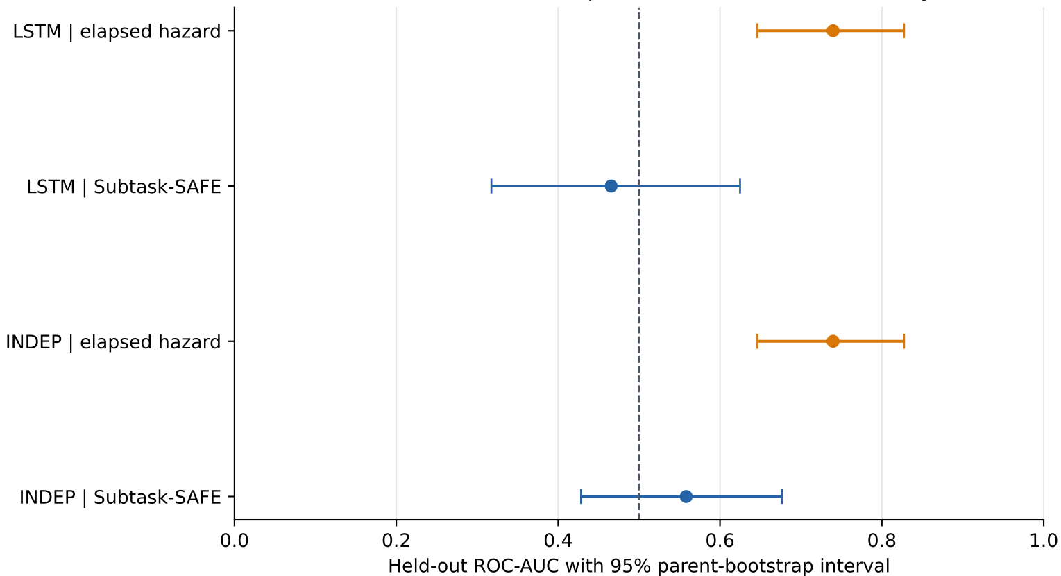
Subtask-SAFE and elapsed-time baseline uncertainty
