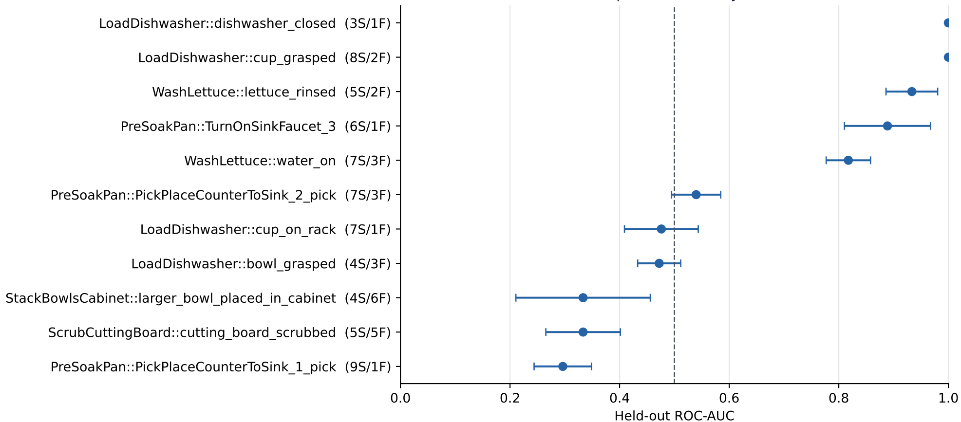
Subtask-SAFE MLP performance by semantic subtask
