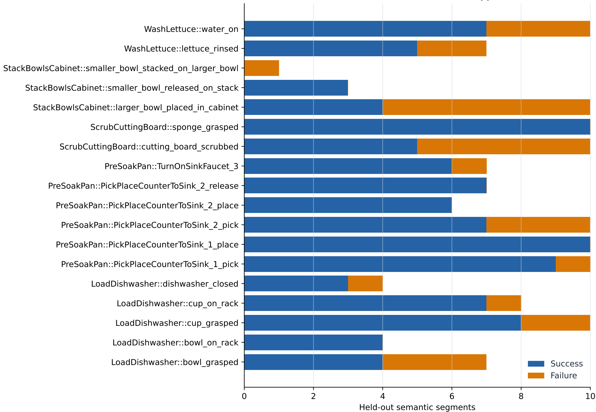
Held-out Subtask-SAFE label support
