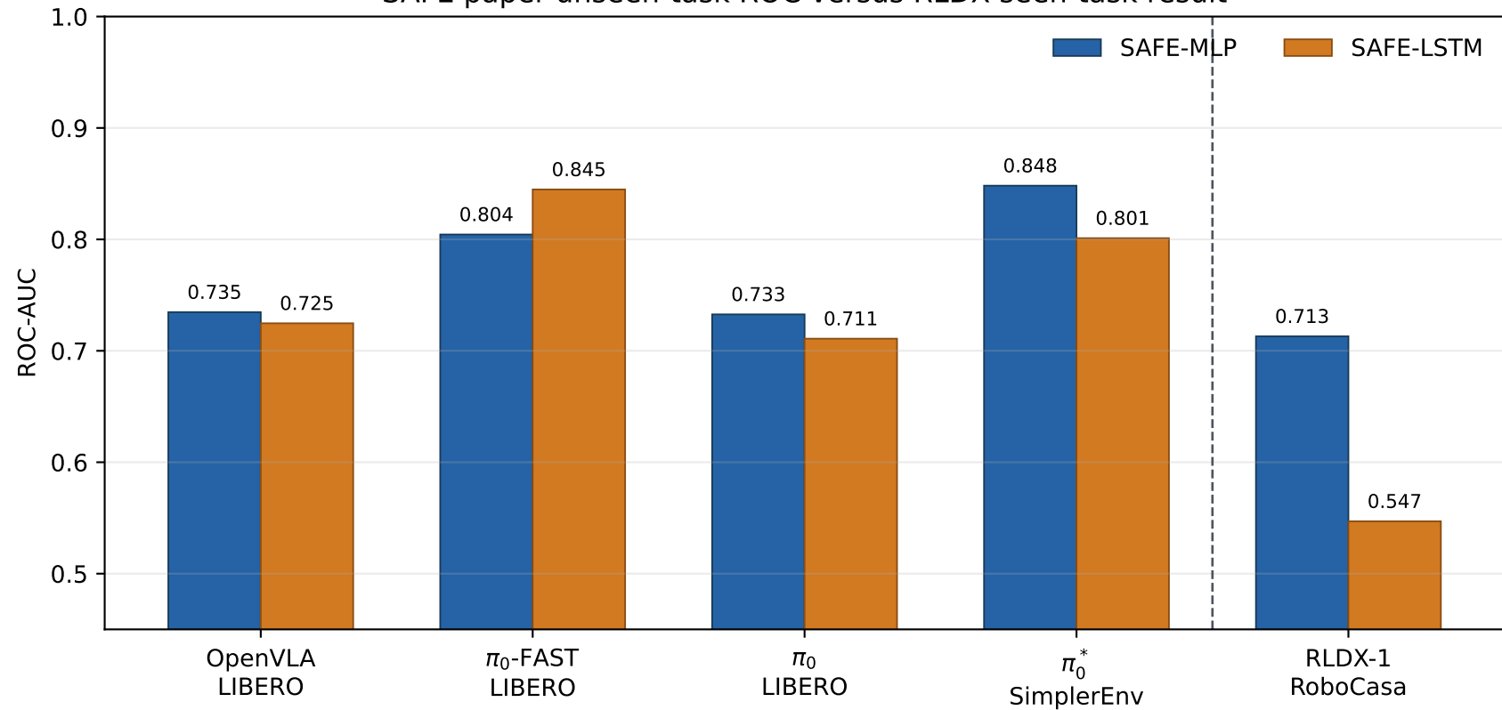
SAFE paper unseen-task ROC versus RLDX seen-task result
