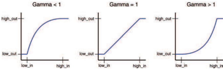
FIGURE 9.12 Gamma transformations for different values of gamma. Redrawn from [GWE04].
