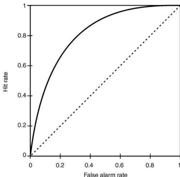
FIGURE 19.5 Example of ROC curve.
