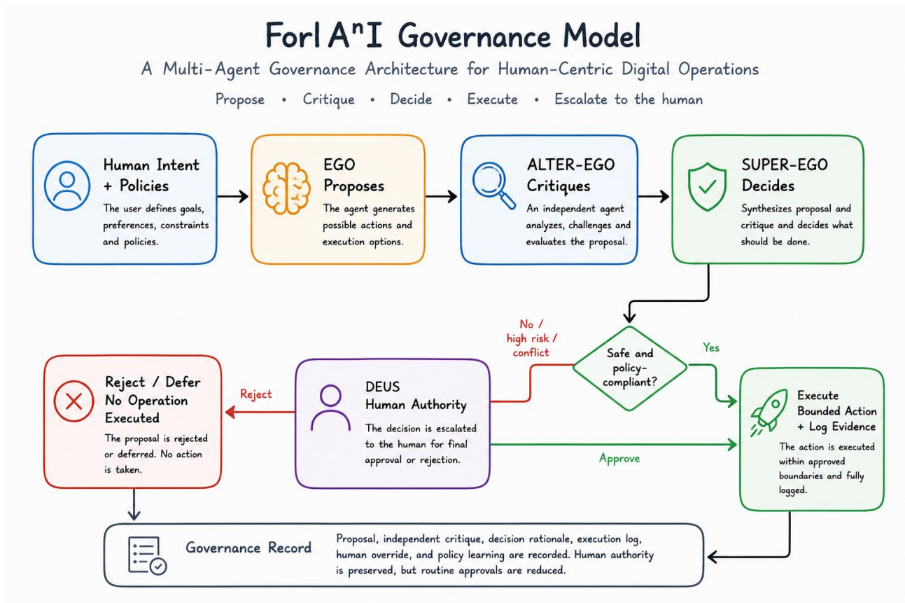
Figure 2. ForlA n I workflow: proposal, critique, synthesis, execution, and escalation.
