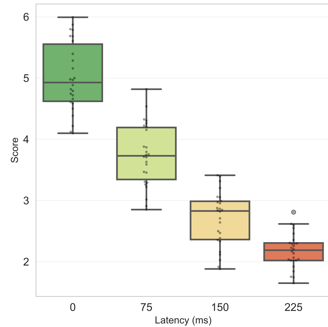
Fitts Law
