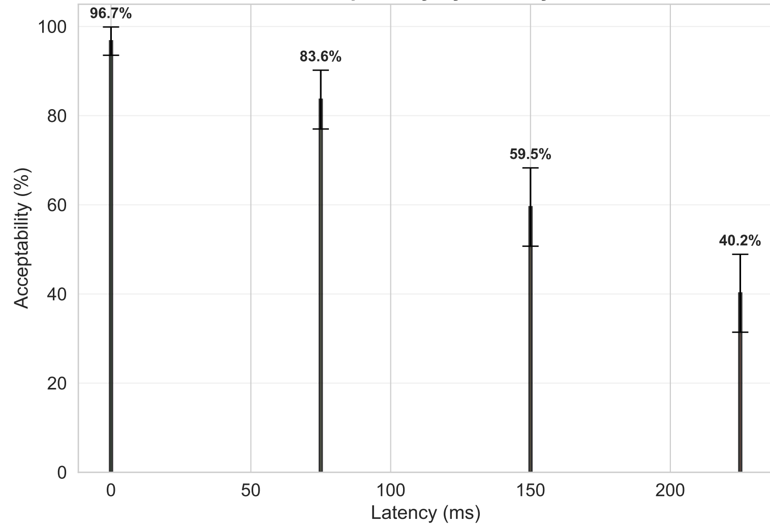
Acceptability by Latency
