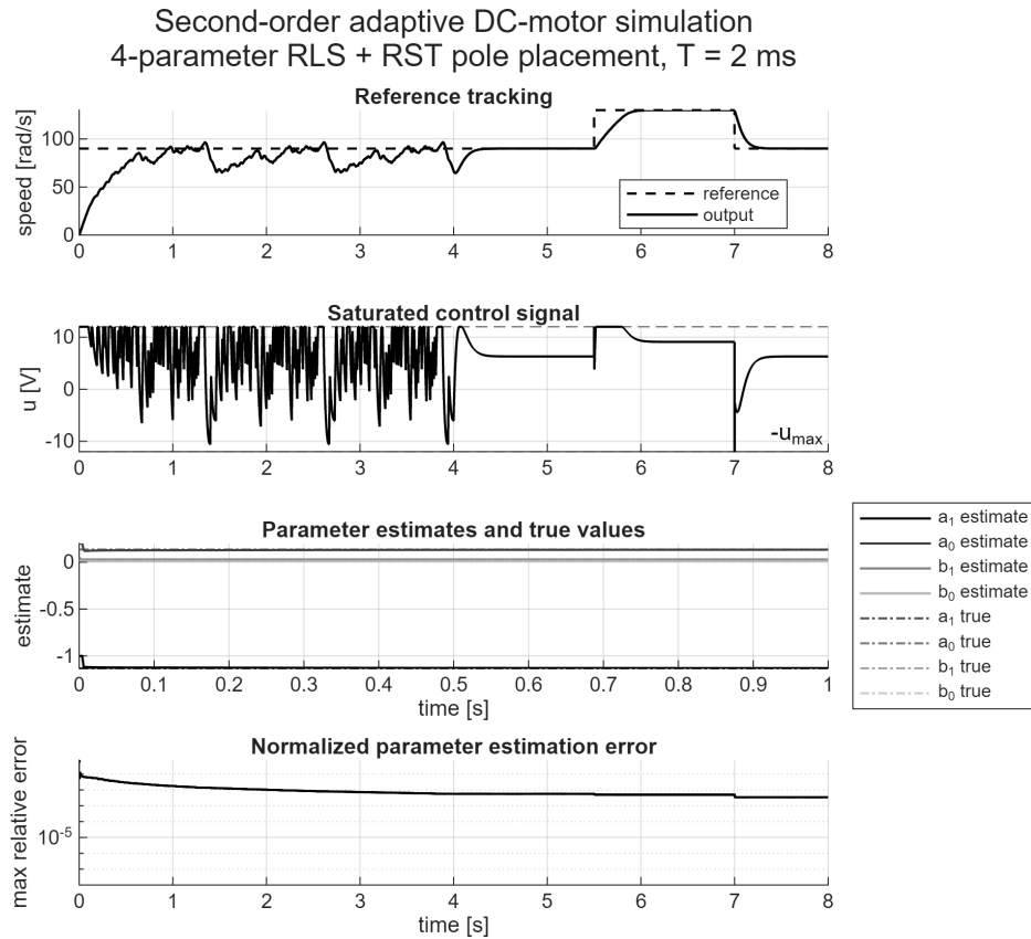
Figure 7.4: Validation run of the second-order adaptive RST controller with T = 2 ms, persistent excitation, integral action, and the electrical pole retained in the desired polynomial.
