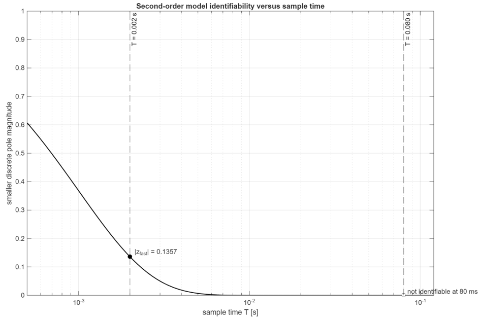
Figure 7.3: Magnitude of the smaller ZOH pole of the second-order motor model as a function of the sampling time.
