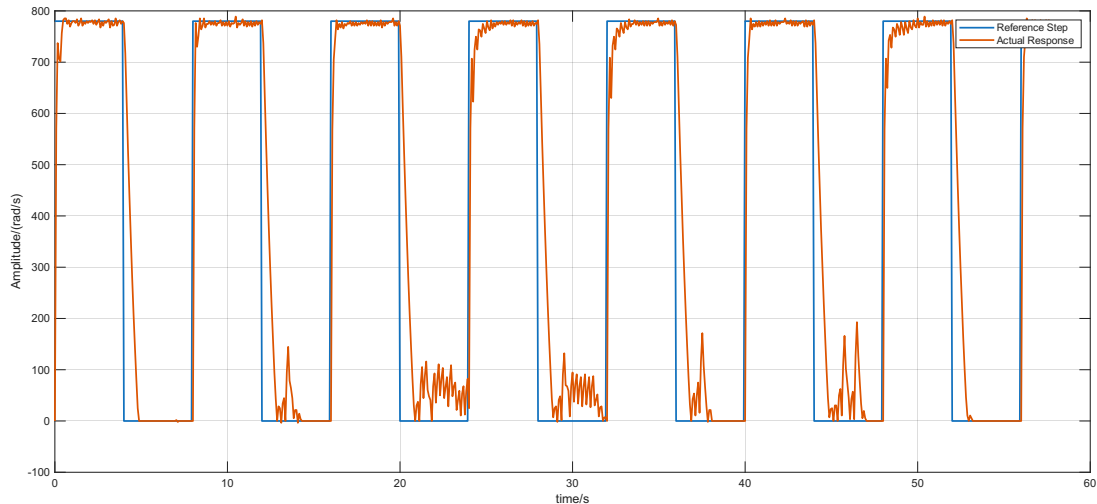
Figure 4: Closed-loop response of the second-order adaptive controller on the hardware rig.
