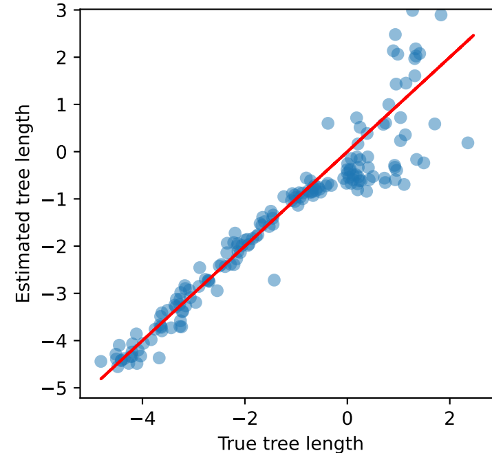
RNN model
