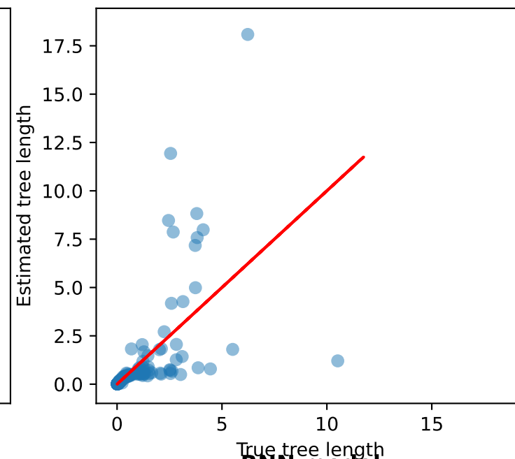
RNN model
