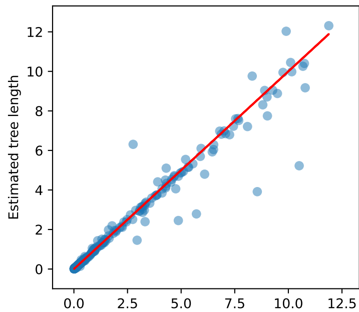
Gamma rate model
