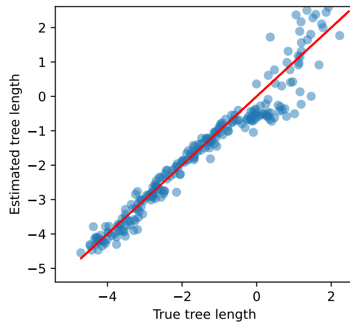
RNN model
