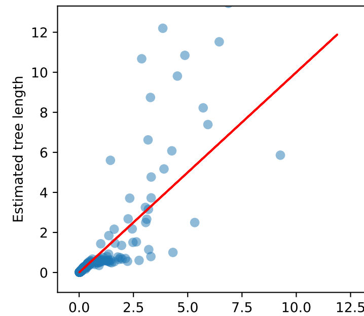
RNN model
