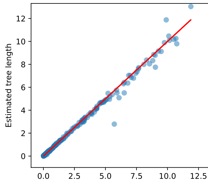
Free rate model
