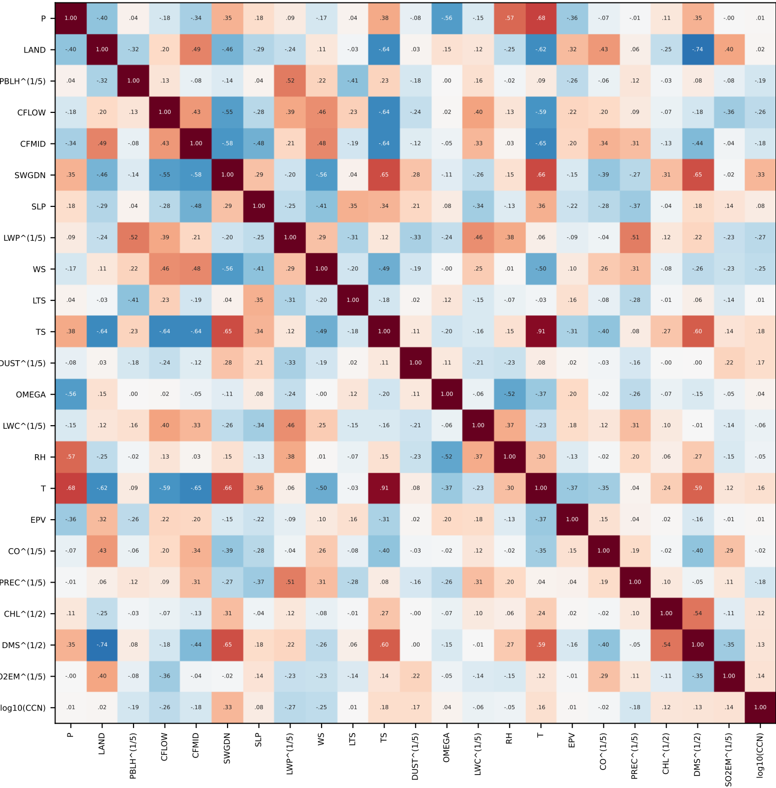
Pearson (linear)
