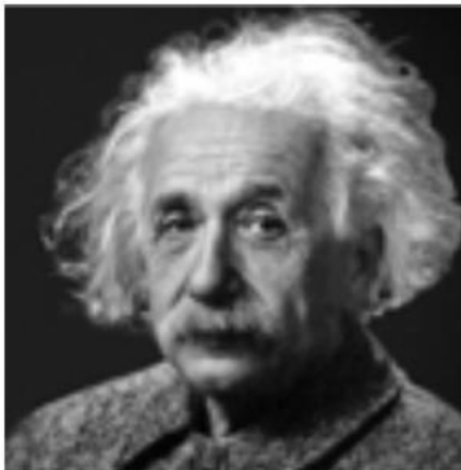
Original Image
