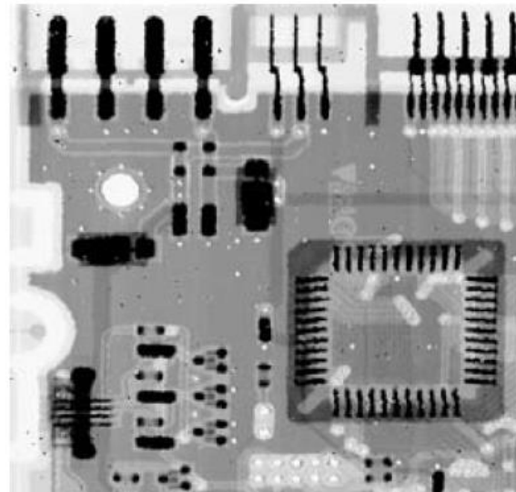
median-filtered ( 3 \times 3 ):
