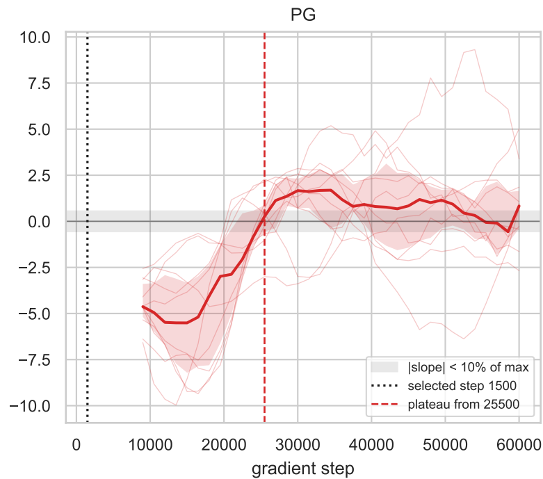
F4 Plateau diagnostic on the validation curve
