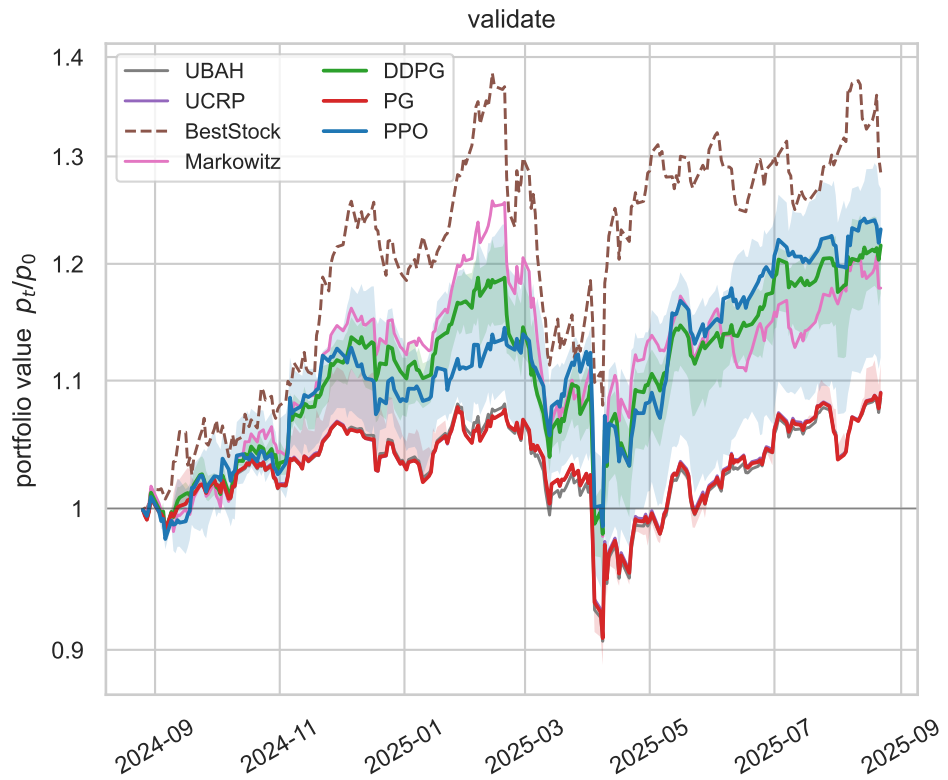
F6 Train and validation wealth
