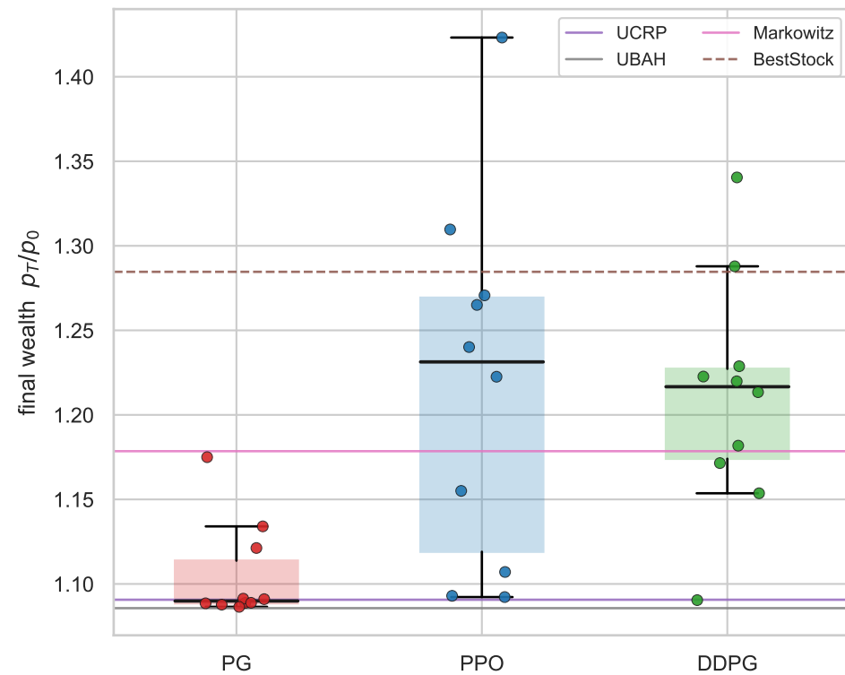
F9 Seed distributions on validate (10 seeds, all shown)
