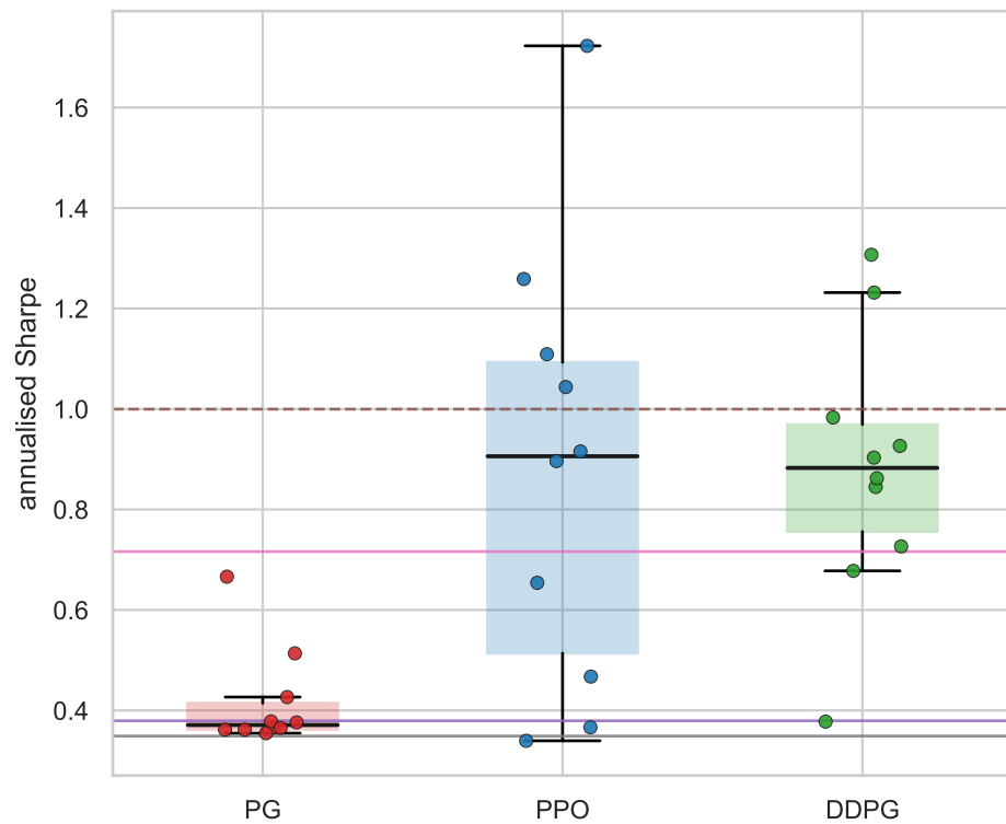
F9 Seed distributions on validate (10 seeds, all shown)
