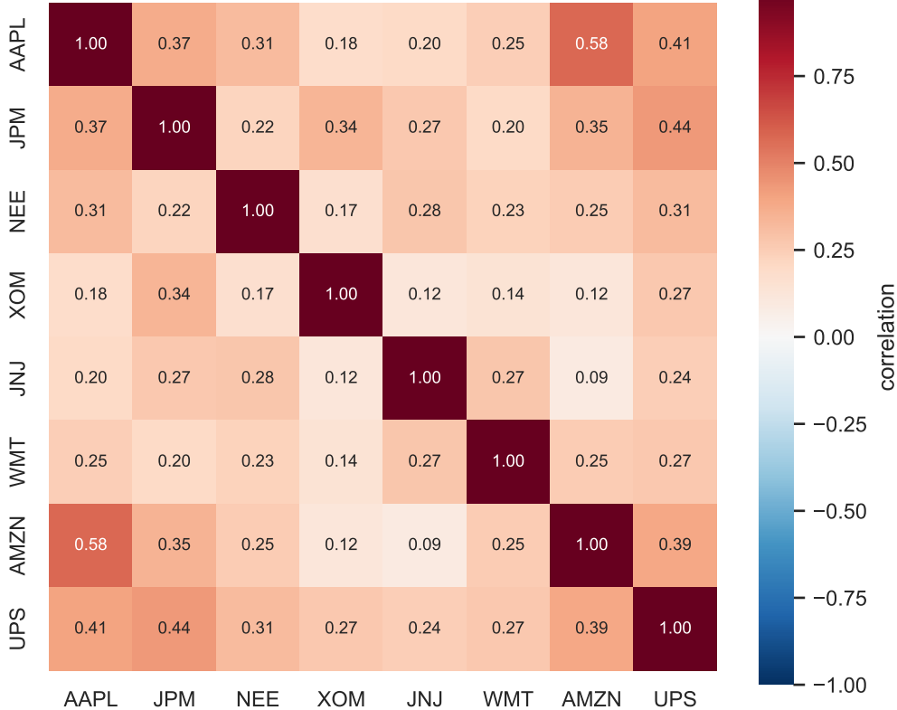
F0b Train-split daily return correlation gate = 0.70 max off-diagonal = 0.576 (AAPL-AMZN)
