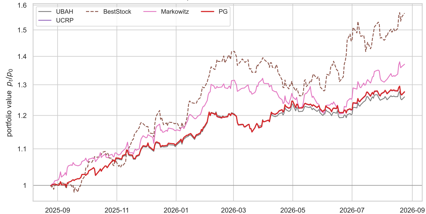
F5 Test-split wealth, net of transaction costs
