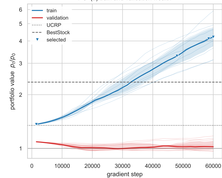
PPO (a) train and validation wealth
