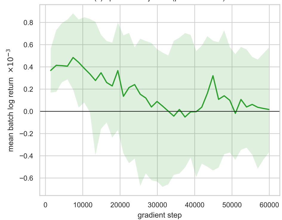
(c) optimised objective (smoothed 2000)
