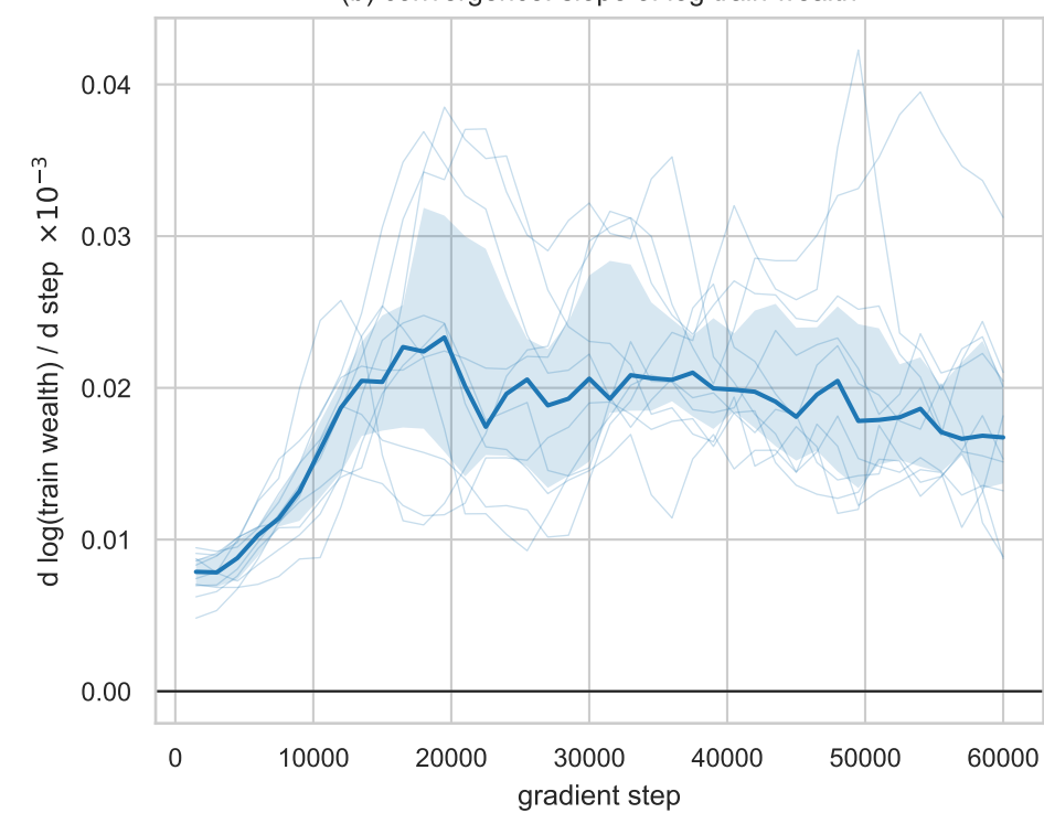
(b) convergence: slope of log train wealth
