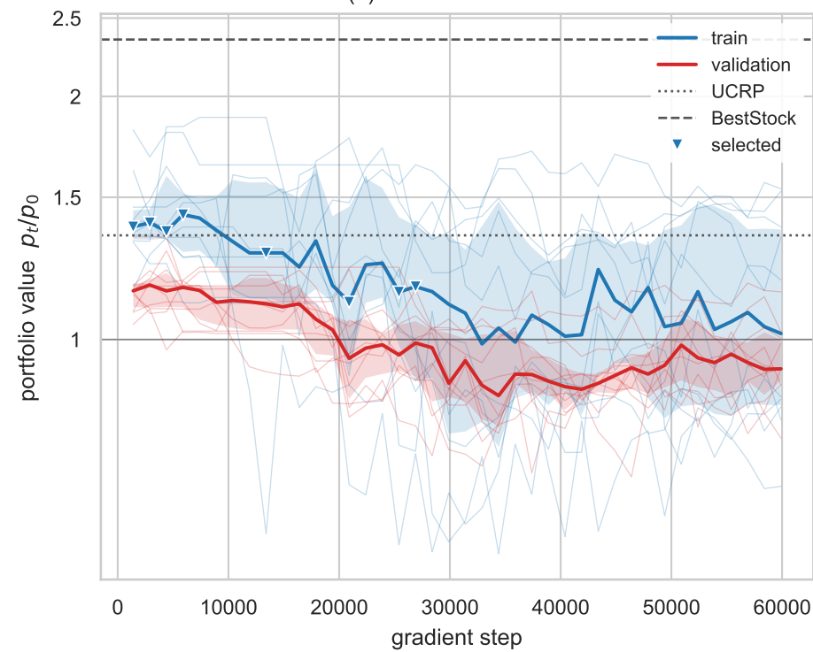
PG (a) train and validation wealth
