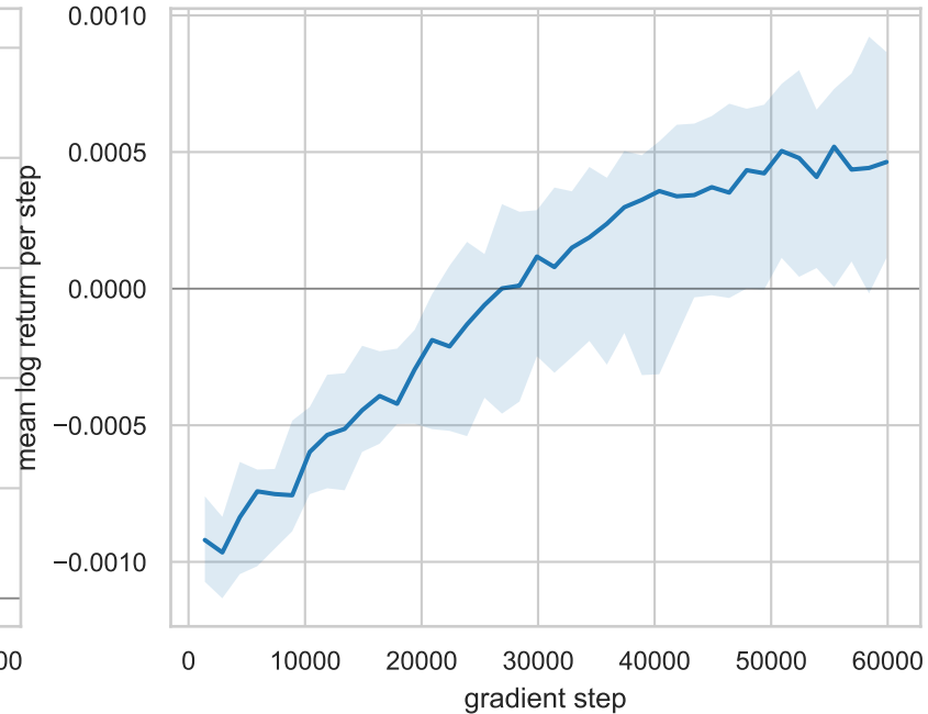
PPO — batch objective (Eq. 21), per evaluation
