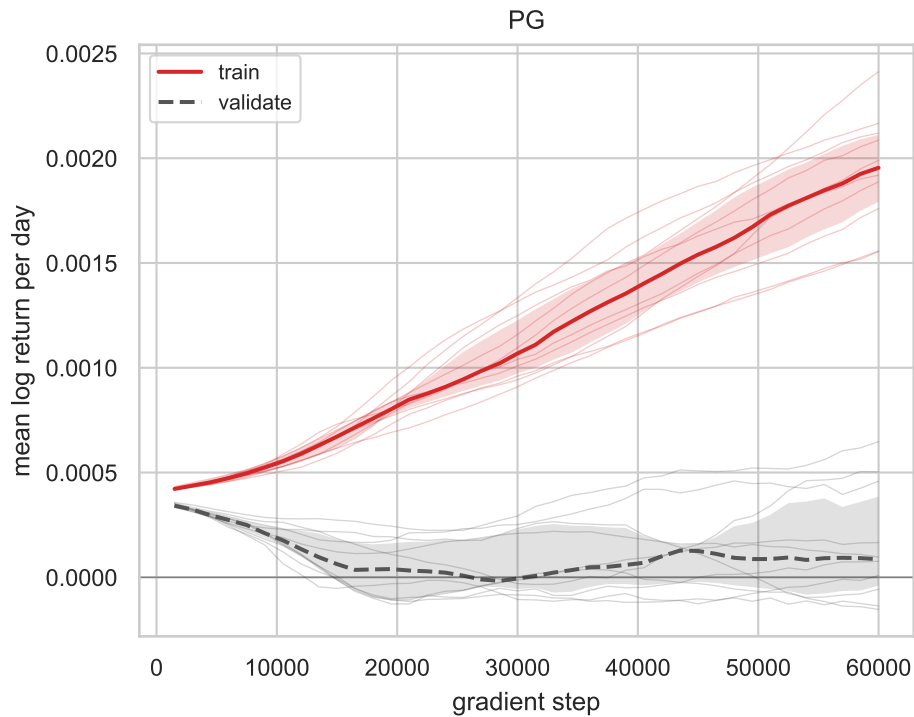
F1 Learning curves (median, IQR, individual seeds)
